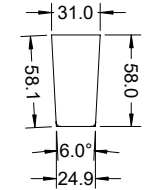
Inside Form
