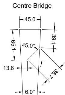
Outside Form
